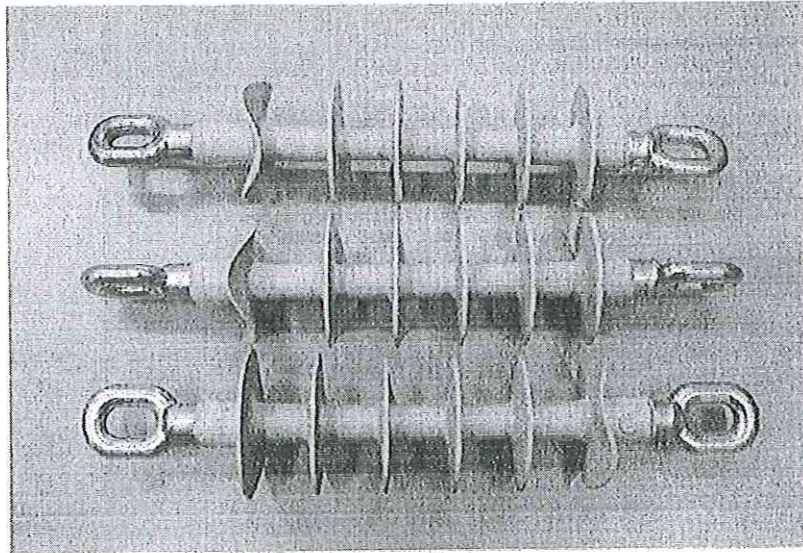
Photo 3 The broken insulators after the tensile failing load test
