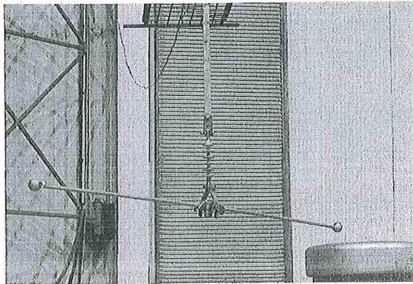
Photo 2 Test arrangement for wet power withstand frequency voltage test
